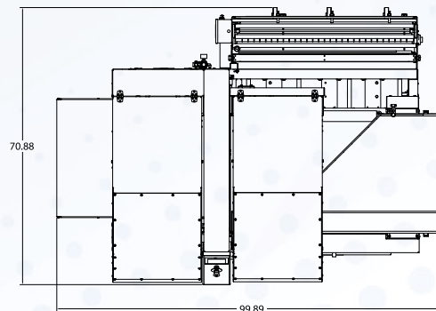
Conflex® FUSION XL Plan View
